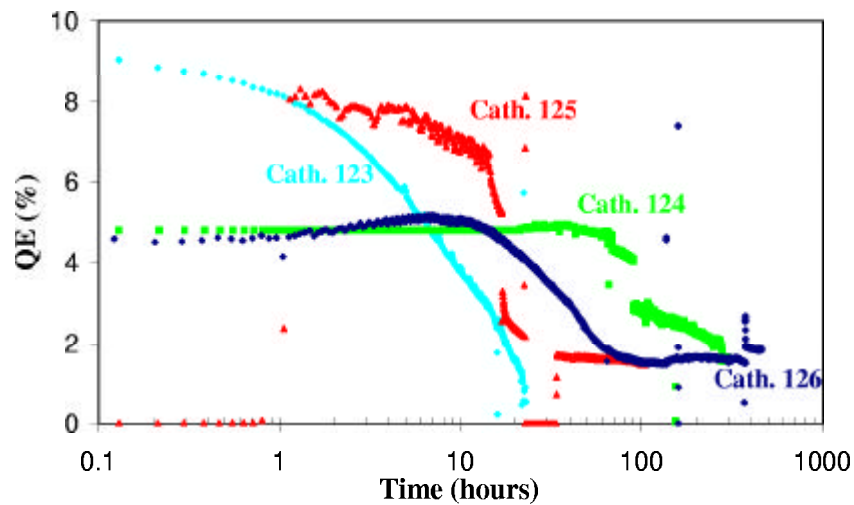
Figure 21: Comparison of the cathodes as a function of time.
